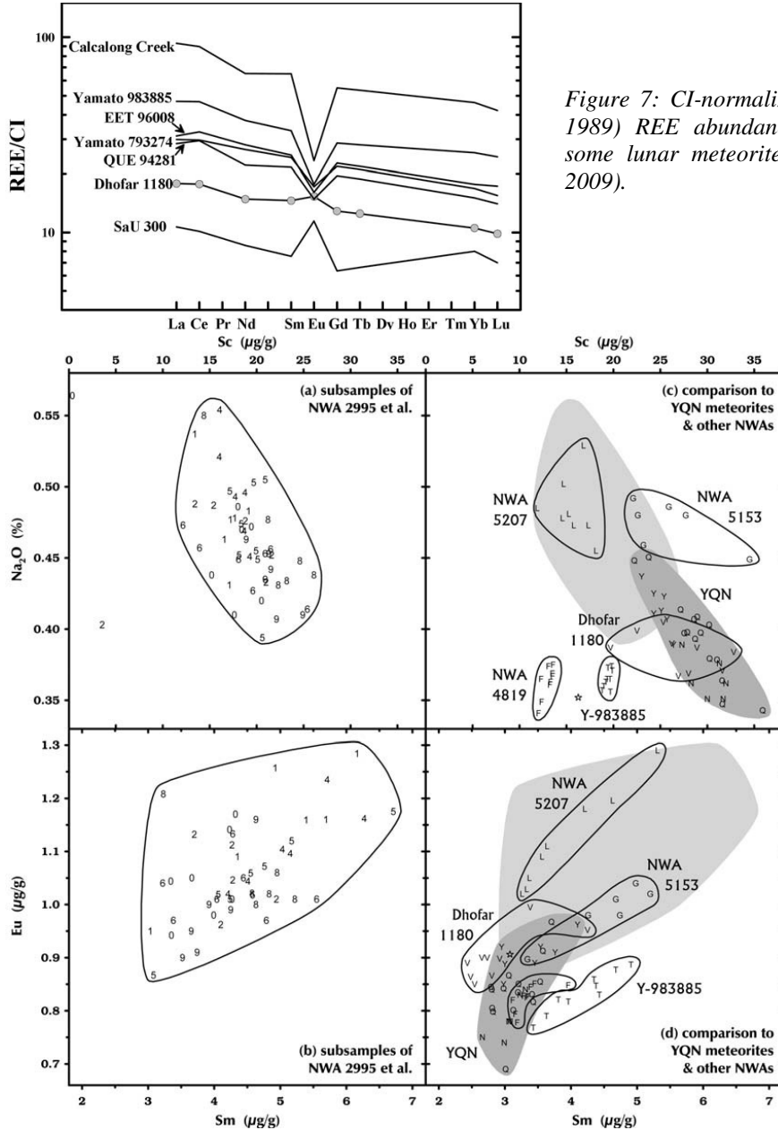
Figure 8: Comparison of Dho 1180 bulk composition to other polymict lunar meteorite breccias, illustrating its distinct composition with slightly higher Eu, lower Sc compared to the YQN pairing group (Yamato, QUE, NWA 2995 pairs; Korotev et al., 2009b).
