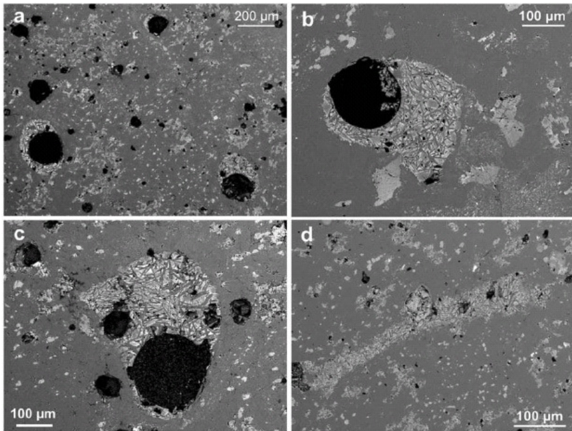
Figure 7: Four backscattered electron images of clasts from Dhofar 026 (and pairs), illustrating a) two typical spheroidal mafic impact melt globules (vesicular) from Dho 461, b) mafic impact melt globule from Dho 465, c) another mafic impact melt globule illustrating a nearly spherical vesicle, within Dho 461, and d) an elongated mafic impact globule from Dho 463 (from Warren et al., 2005).
