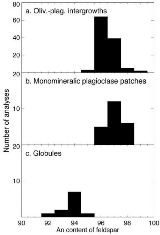
Figure 8: Feldspar compositions from intergrowths, globules and monomineralic areas in Dhofar 026 (from Cohen et al., 2004).
