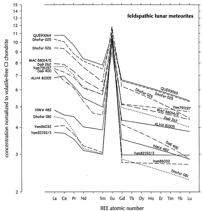
Figure 11: REE concentrations for Dho 026 compared to those for other lunar feldspathic meteorites (from Korotev et al., 2003).
