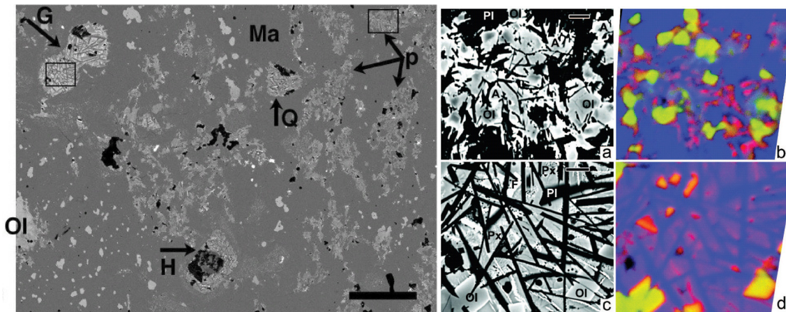
Figure 6: Back scattered electron image of a region of Dhofar 026 (left) illustrating the textures in this breccia, as well as highlighting several of the clast textures observed by Cohen et al. (2004) and Warren et al. (2005). Top right images (a and b) are from a pyroxene-plagioclase intergrowth (top right corner of left hand BSE image), and bottom right images (c and d) are from an ovoid globule (G in left hand image).
