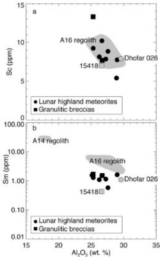
Figure 9: Sc and Sm (ppm) vs. Al_2O_3 for some lunar highlands meteorites including Dhofar 026 and also granulitic breccias (from Cohen et al., 2004).
