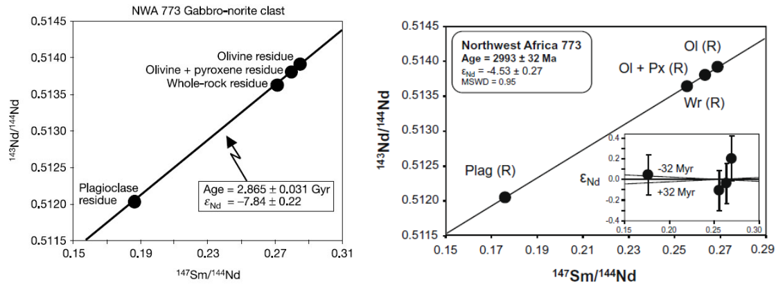
Figure 15: (left) Sm-Nd isochron for gabbro whole rock and mineral separates (from Borg et al., 2004) (right) Sm-Nd isochron for gabbro whole rock and mineral separates (from Borg et al., 2009). The revised age for NWA 773 makes it older than NWA 032 and therefore not the youngest dated lunar sample as argued in the earlier work by Borg et al. (2004).
