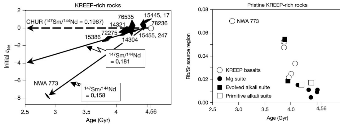
Figure 16: Sm-Nd modeling of source region for NWA 773 indicates derivation from the most LREE enriched (low epsilon Nd) source known for lunar materials (from Borg et al., 2004).
