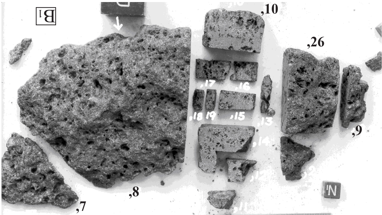
Figure 14: Group photo after cutting slab from 71055. Small cube is 1 cm. NASA S73-34148. This is the top, exposed lunar surface.
