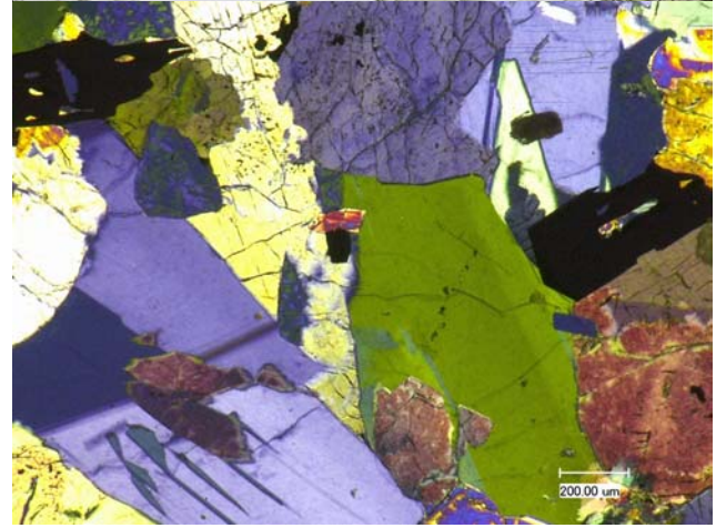
Figure 2d: Photomicrograph of thin section 12064,8 by C Meyer @ 100x (bottom is with crossed polarizers).
