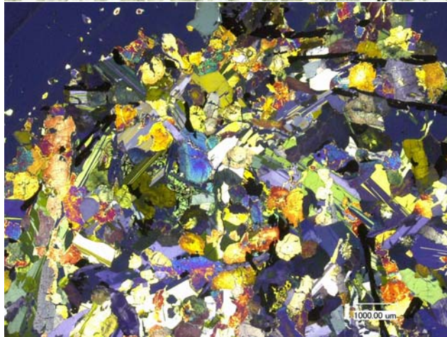
Figure 2c: Photomicrograph of thin section 12064,8 by C Meyer @ 30x.
