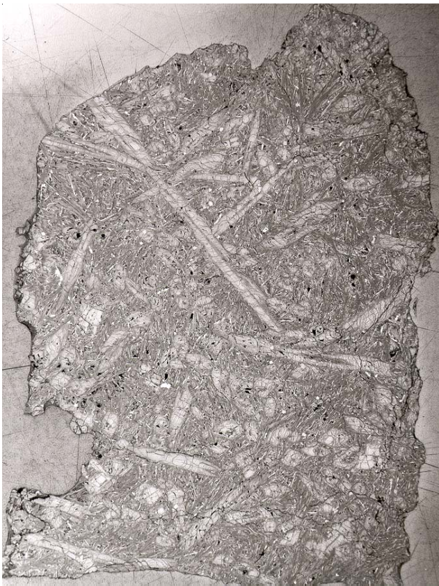
Figure 2a: Reflected light photo of thin section 12052,6. Scale about 3 cm. NASA #S70-30232.
