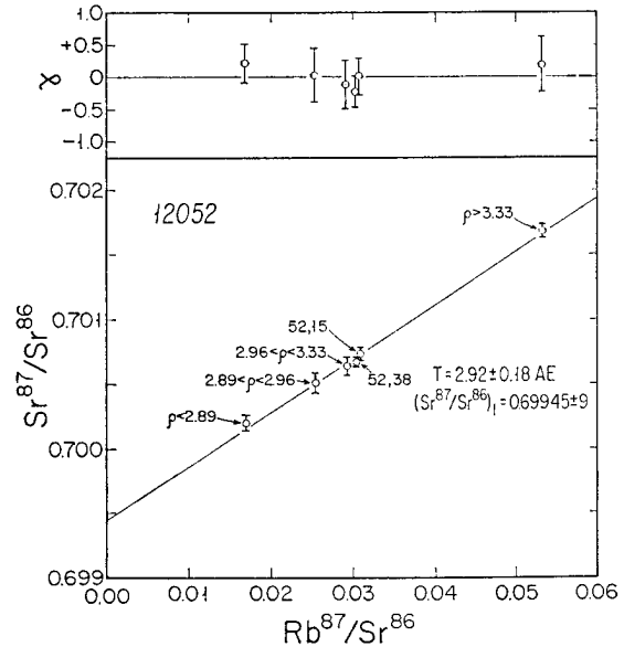
Figure 8: Rb/Sr isochron for 12052 (from Murthy et al 1971).
