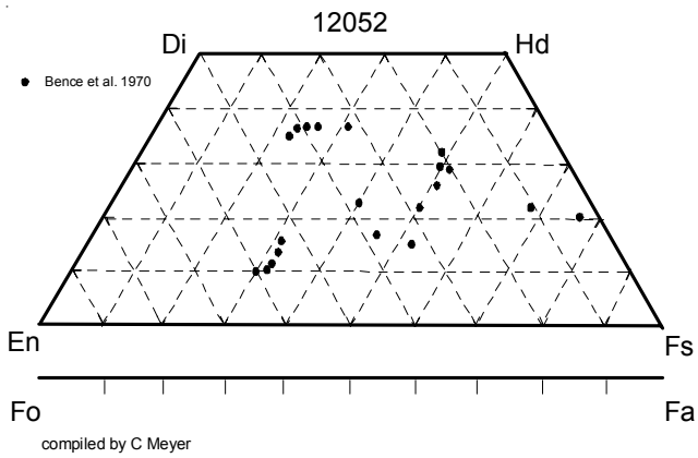
Figure 4: Bence et al. (1970, 1971) determined the composition of pyroxene in 12052.
