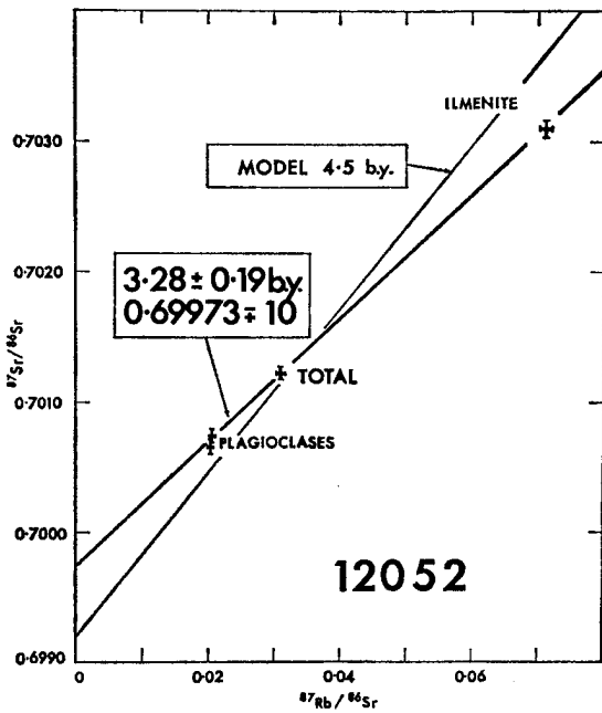
Figure 7: Rb/Sr isochron diagram for 12052 (from Compston et al. 1971).
