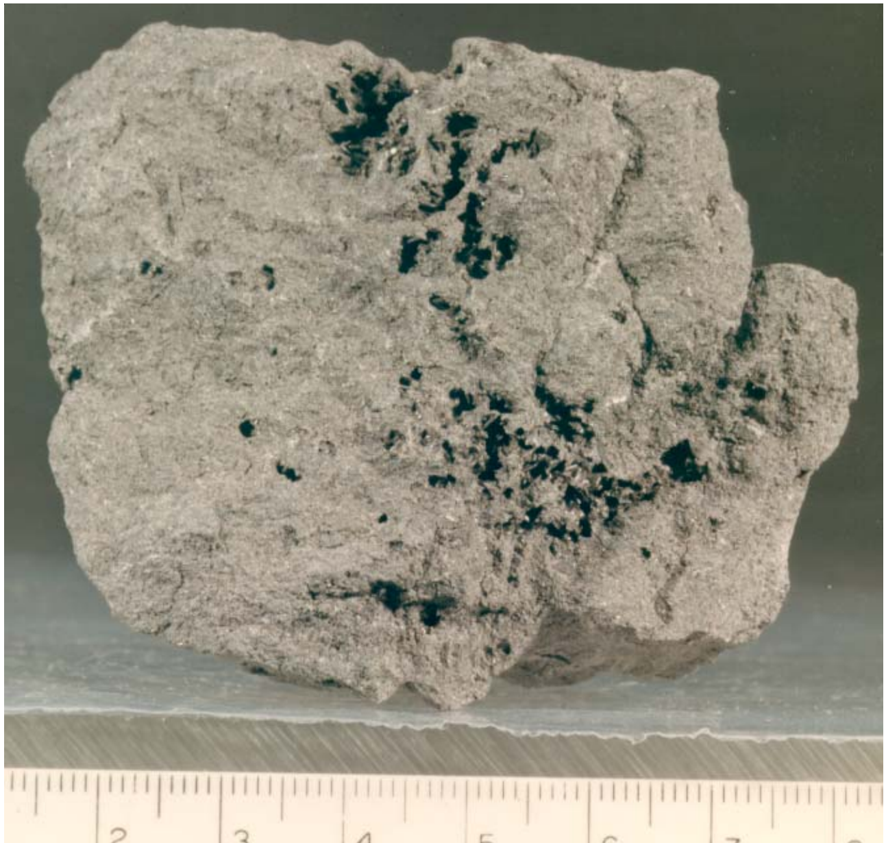
Figure 9: Photo of broken surface of 12052,1 showing pyroxene crystals in vugs. NASA #S70-44847. Scale 1 cm.
