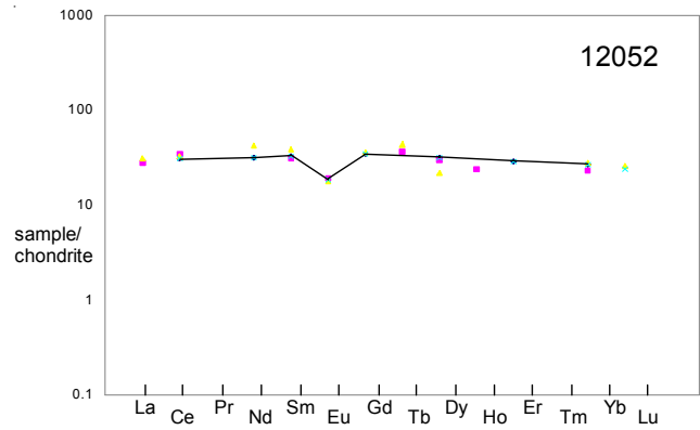
Figure 5: Normalized rare-earth-element diagram for 12052 (data from Wanke et al. connected).
