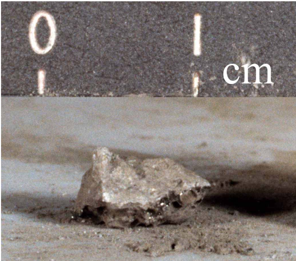
Figure 1. Sample 15336. The vesicular glass is on the bottom on this view. S-71-49633
